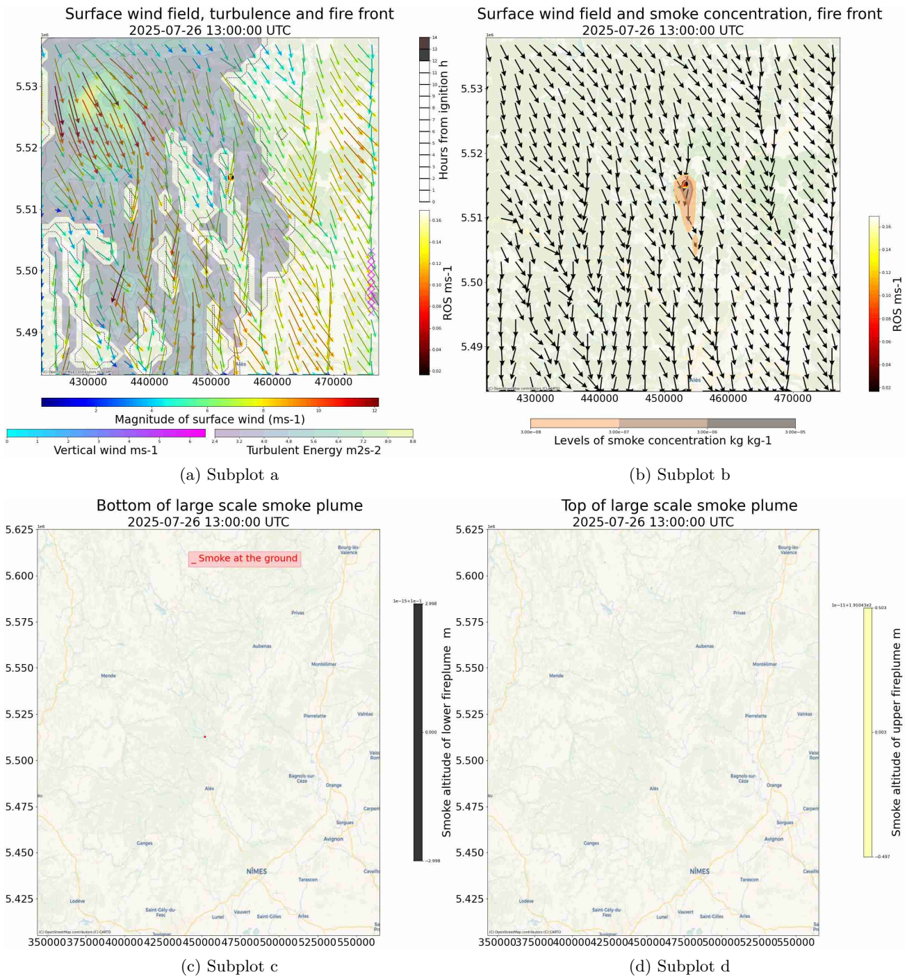
Figure 1: 2025-07-26T14:00:00Z
