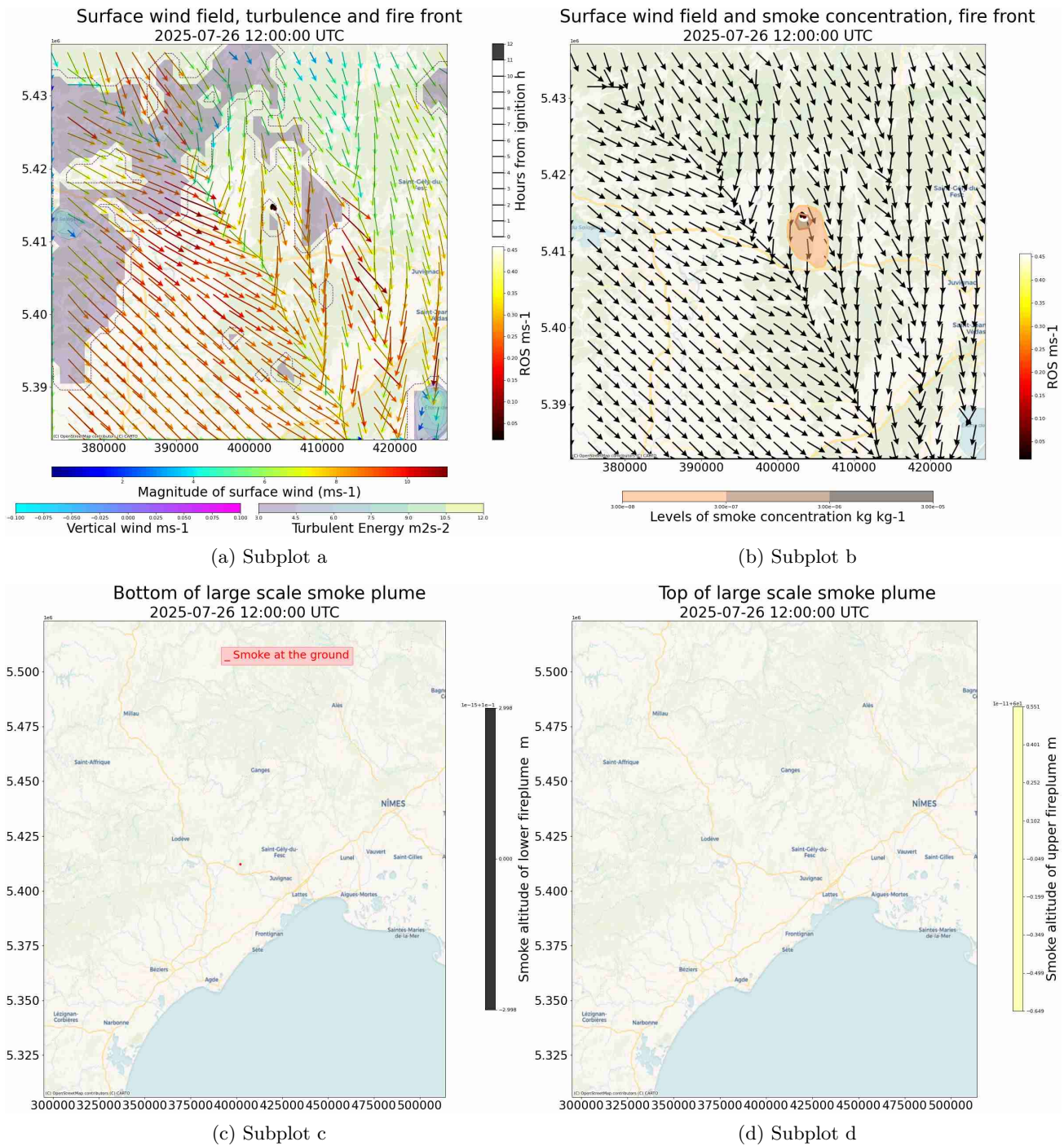
Figure 1: 2025-07-26T13:00:00Z
