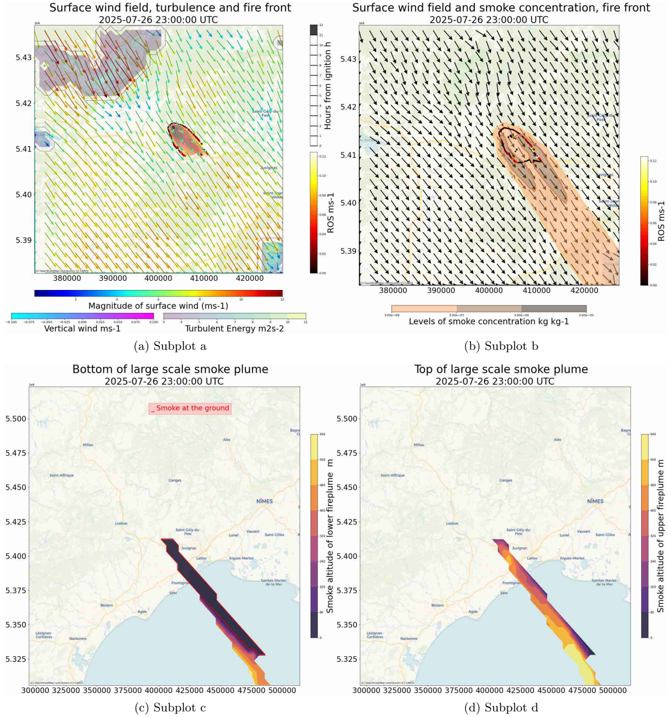
Figure 12: 12025-07-26T14:00:00Z
