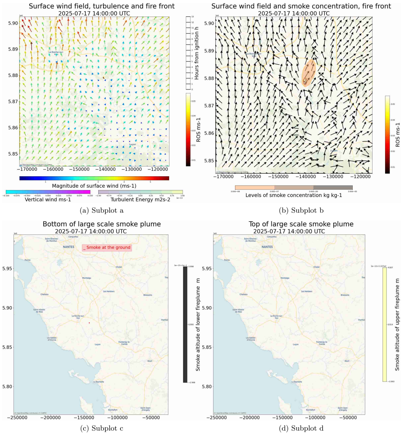
Figure 1: 2025-07-17T15:00:00Z
