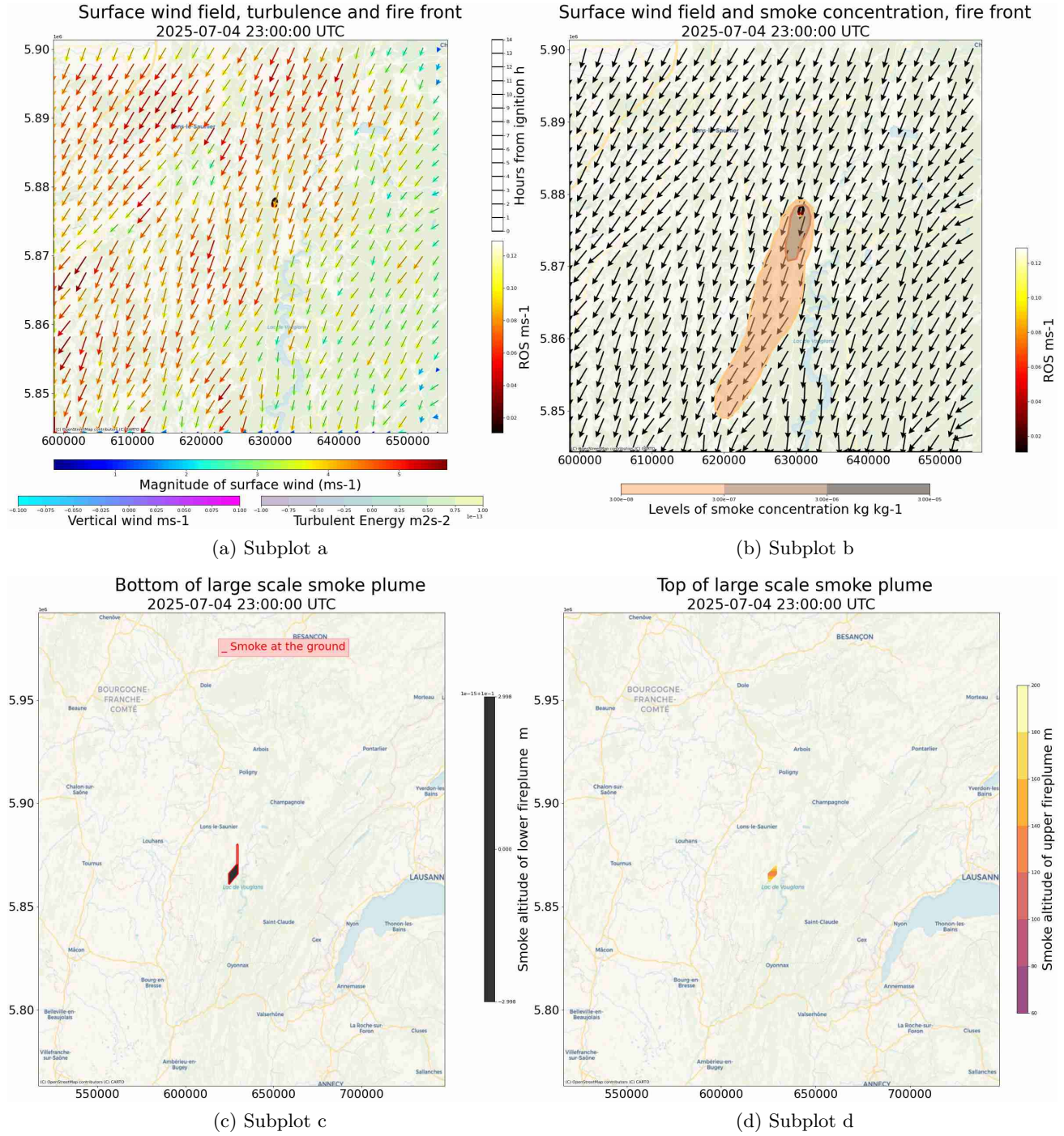
Figure 2: 2HAFTERSTARTFIRE
