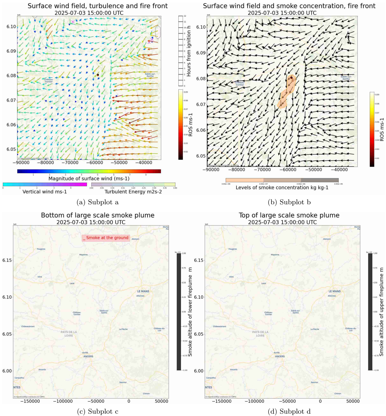
Figure 1: 2025-07-03T16:00:00Z
