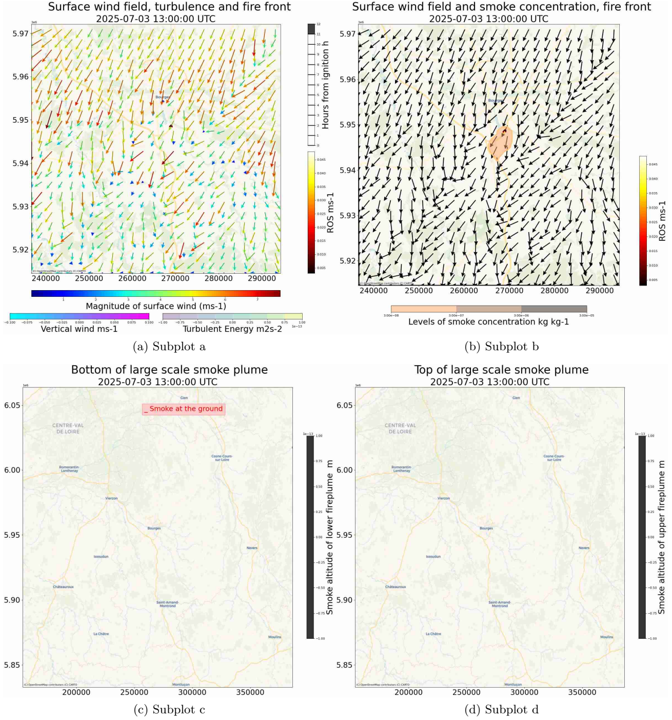
Figure 2: 2025-07-03T14:00:00Z
