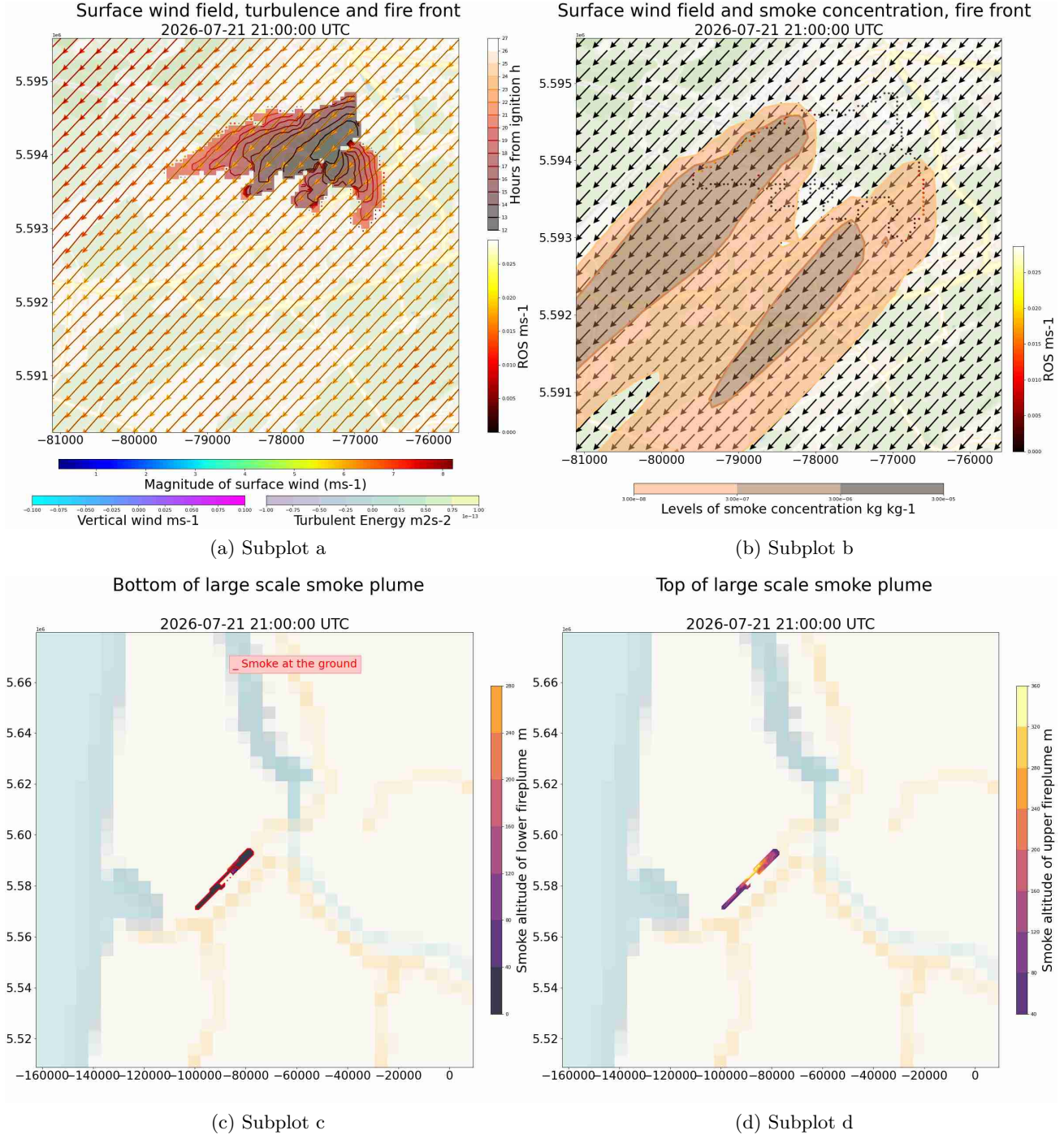
Figure 9: 2026-07-21T22:00:00Z
