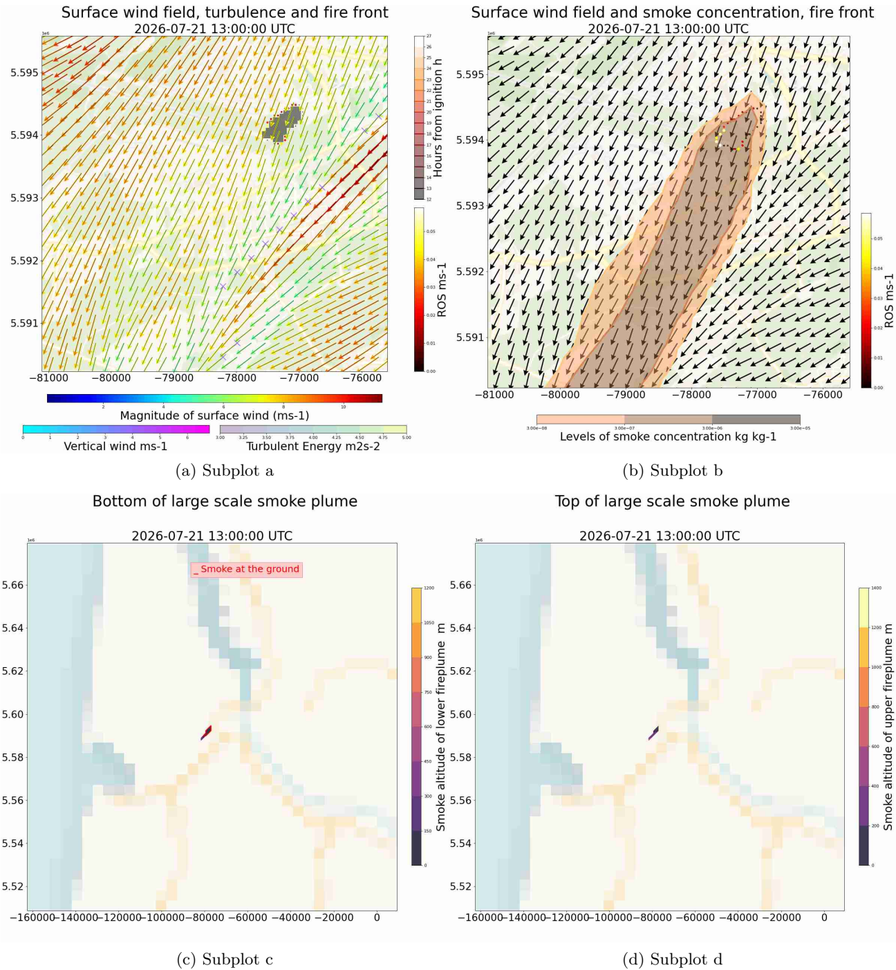
Figure 1: 2026-07-21T14:00:00Z
