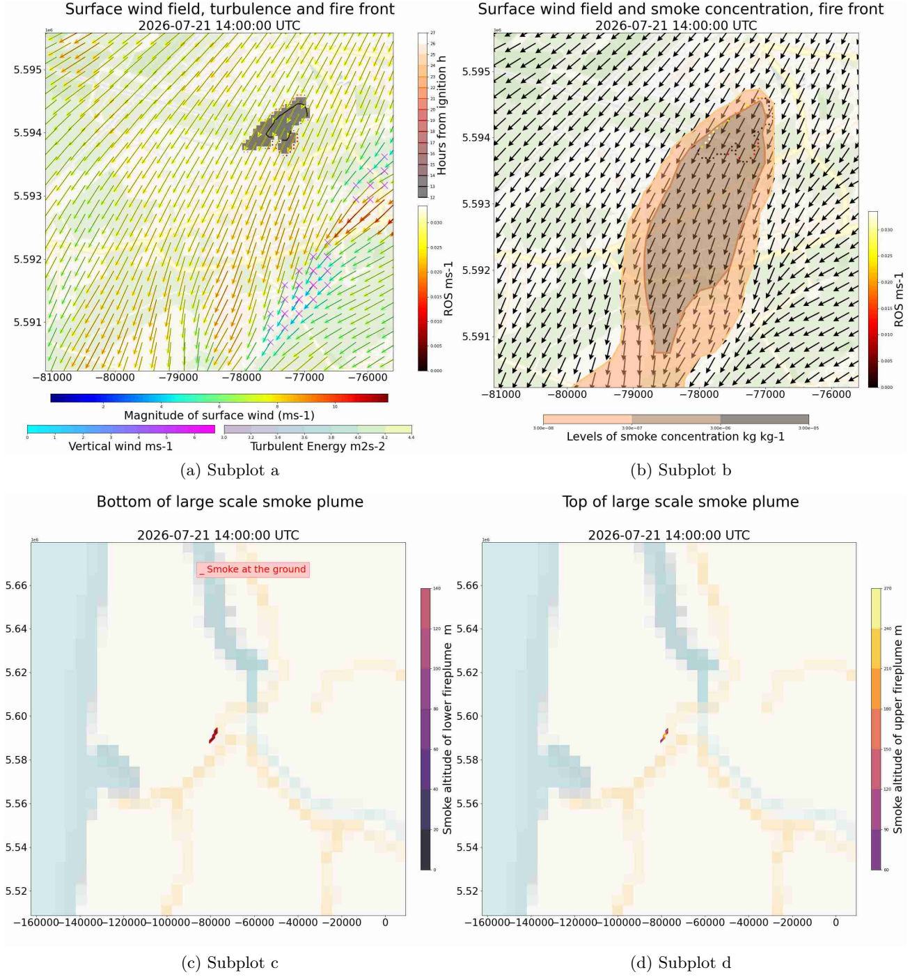
Figure 2: 2026-07-21T15:00:00Z
