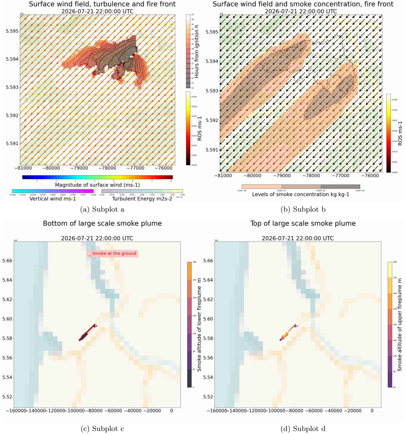
Figure 10: 2026-07-21T23:00:00Z
