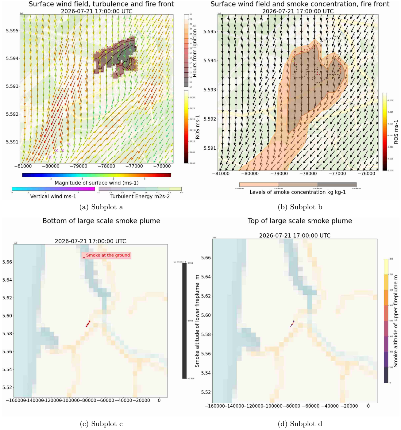
Figure 5: 2026-07-21T18:00:00Z
