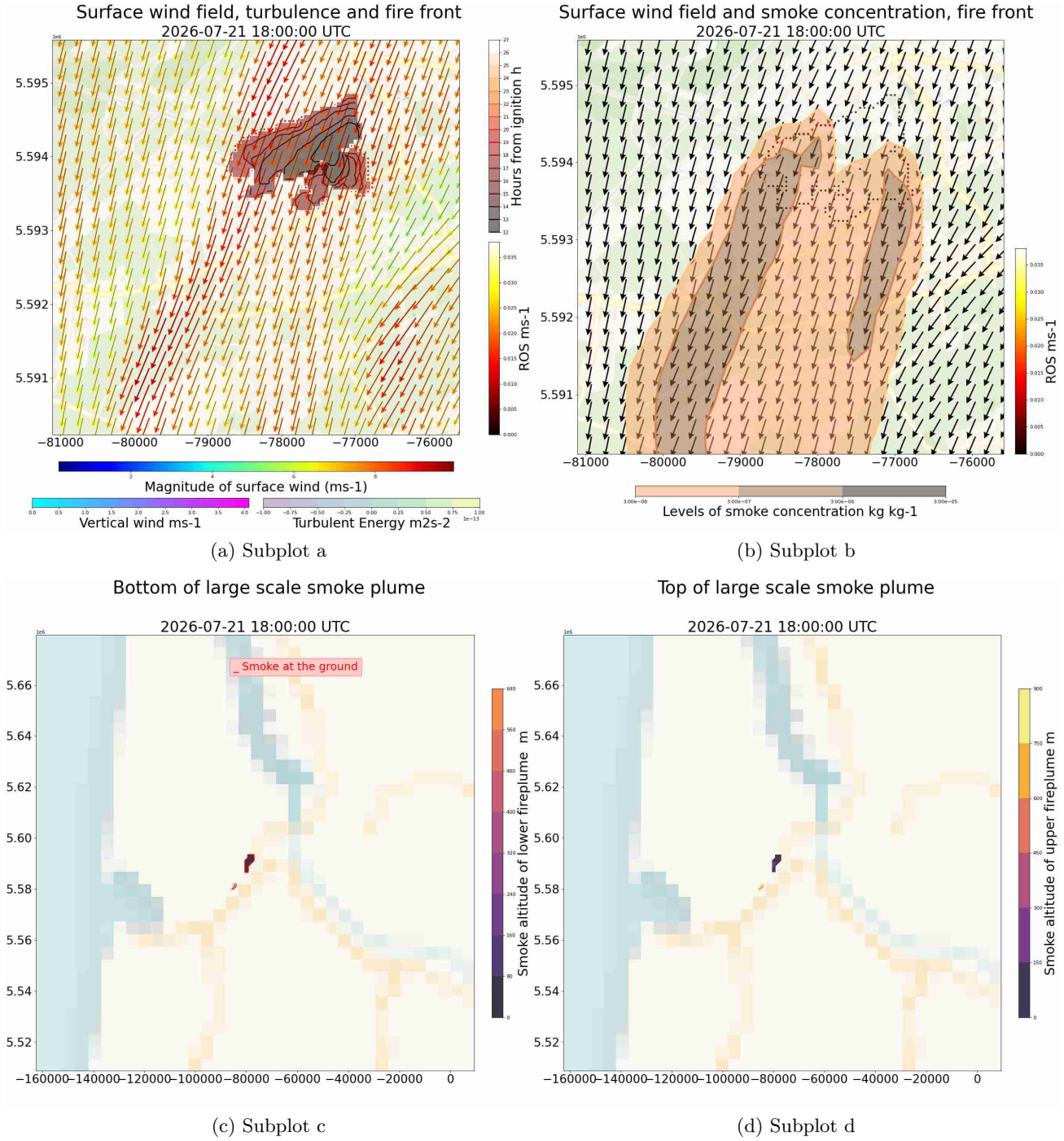
Figure 6: 2026-07-21T19:00:00Z
