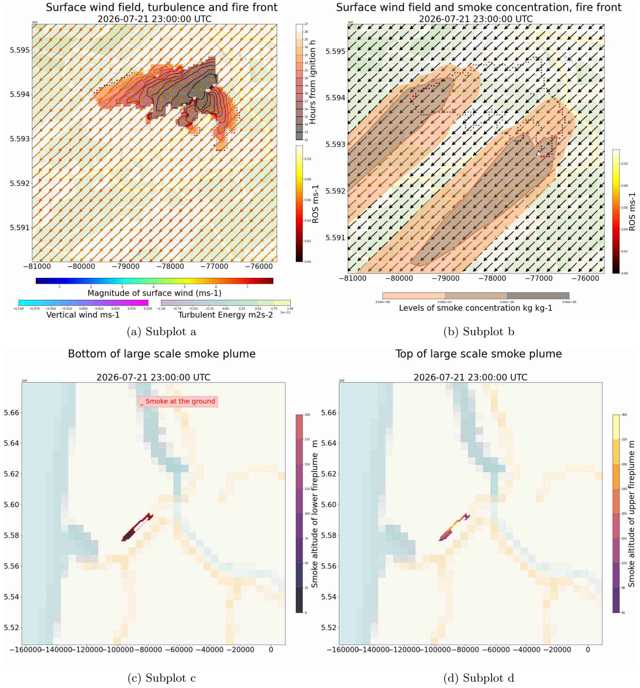
Figure 11: 12026-07-21T14:00:00Z
