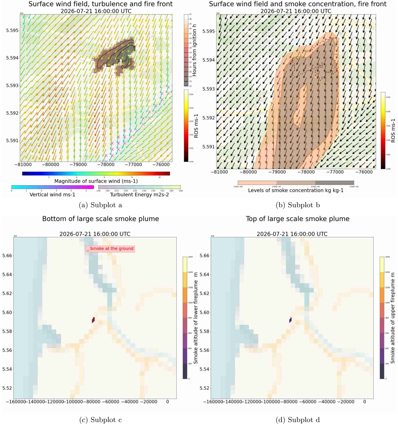
Figure 4: 2026-07-21T17:00:00Z
