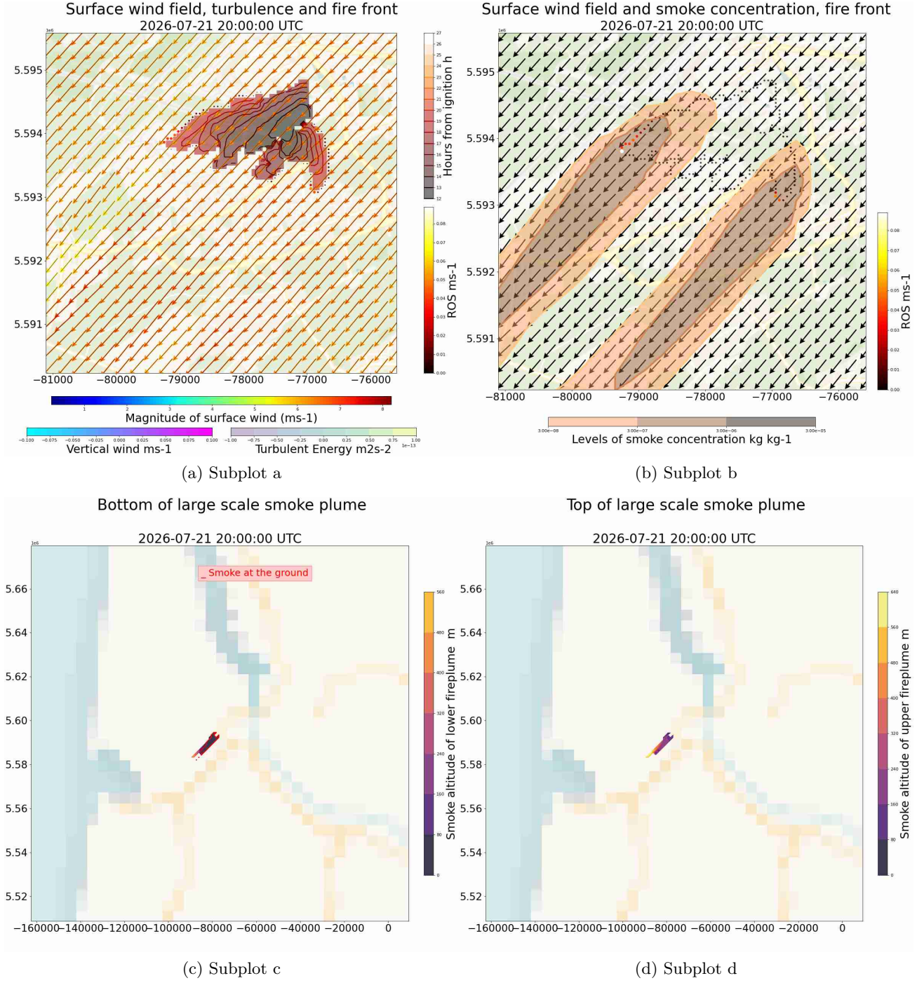
Figure 8: 2026-07-21T21:00:00Z
