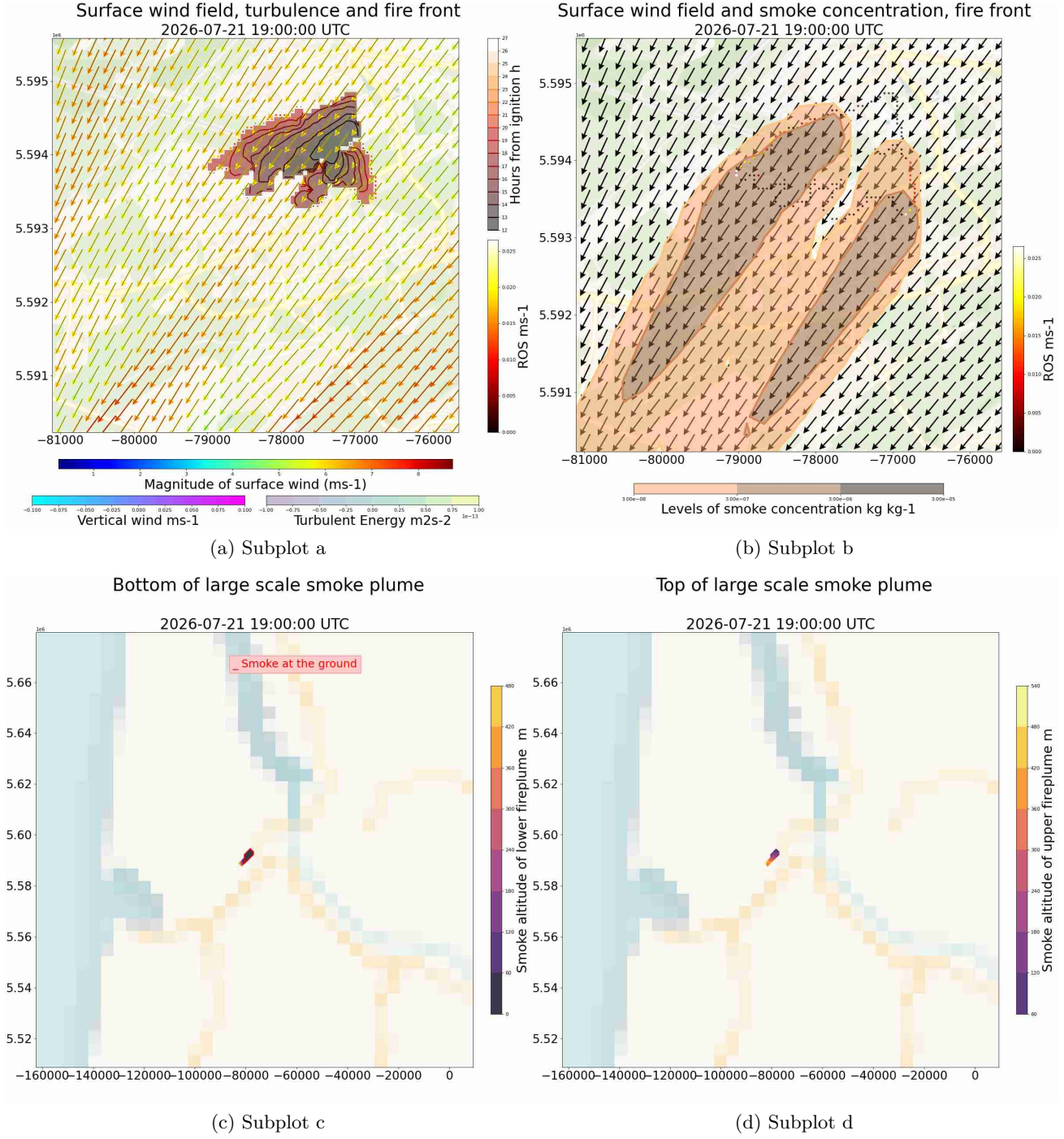
Figure 7: 2026-07-21T20:00:00Z
